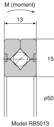
Cross-Roller Ring
